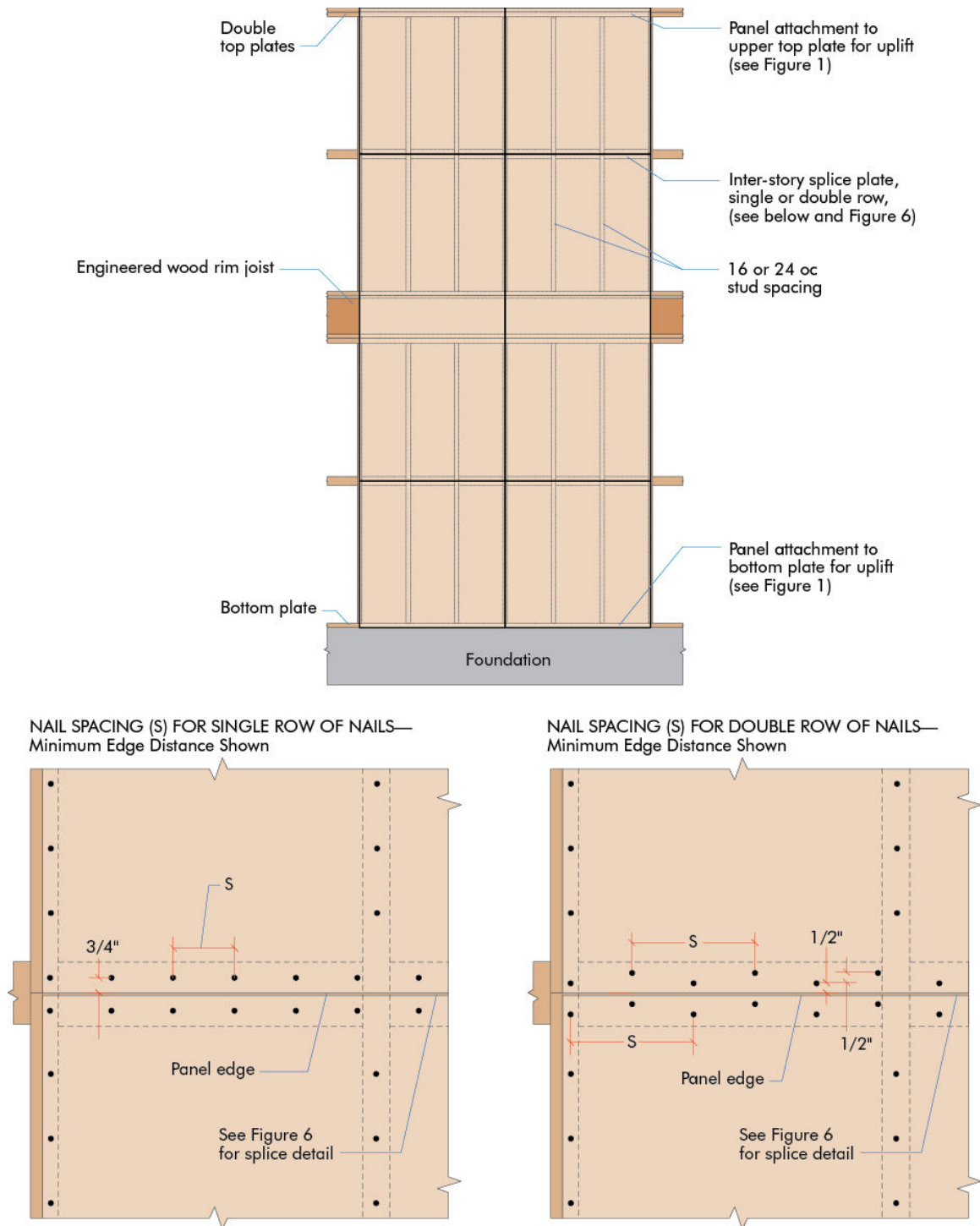
Figure 3. Panel attachment for shear and uplift at inter-story splice plate
